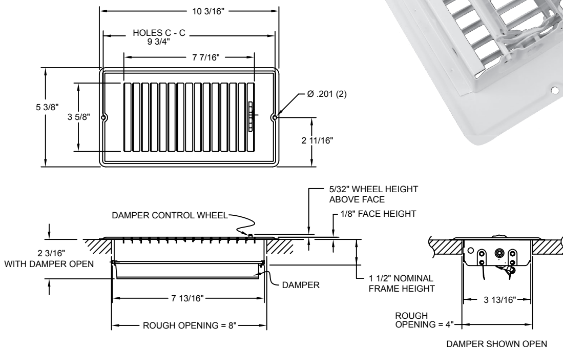
DAMPER SHOWN OPEN
