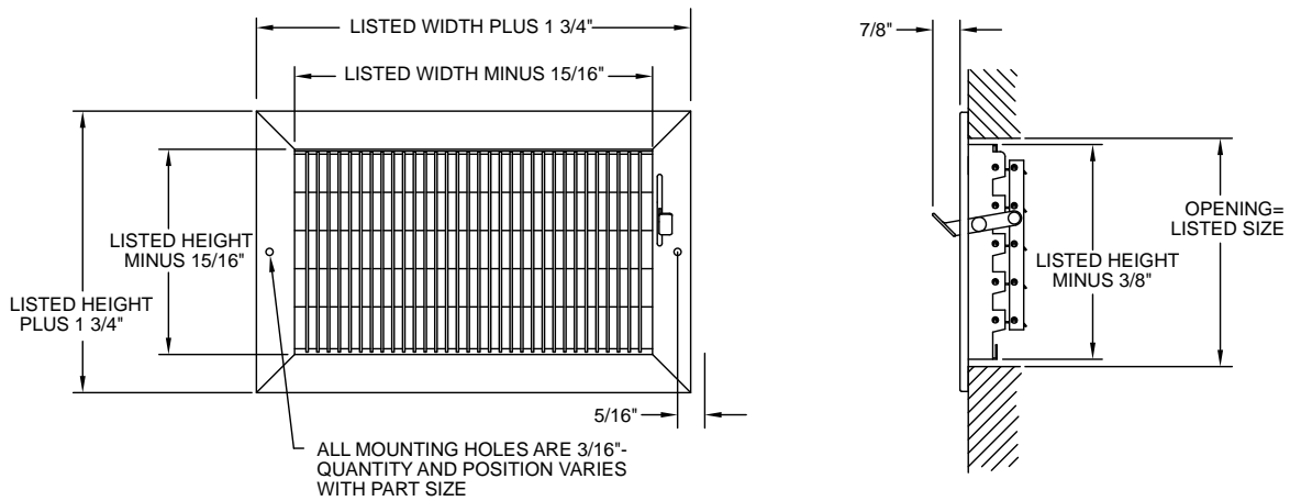
DAMPERS SHOWN OPEN, ALL VIEWS
