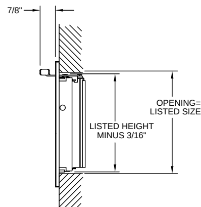
DAMPERS SHOWN OPEN, ALL VIEWS
