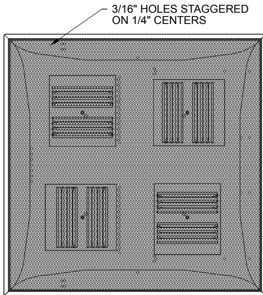
WITH OPTIONAL 4-WAY DIFFUSER
