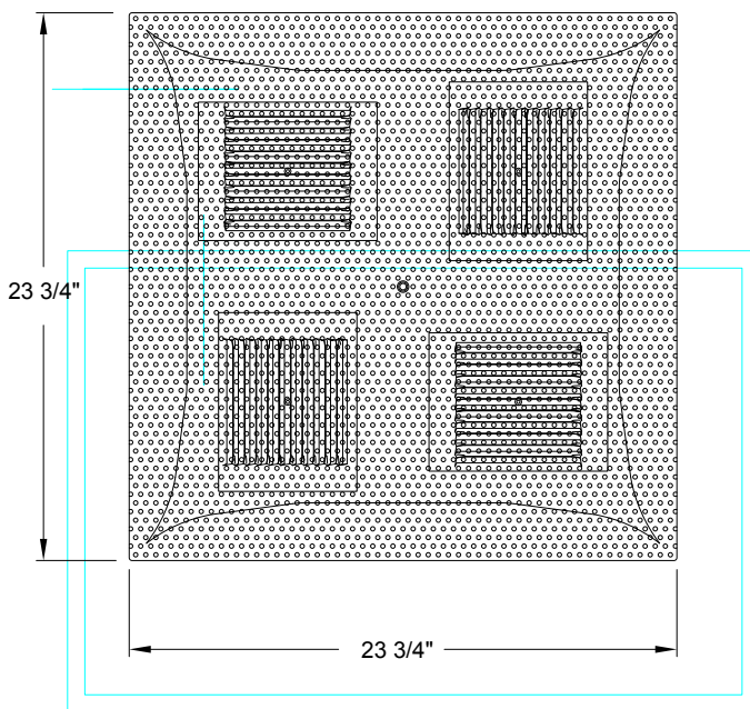
PDSWD SERIES, PERFORATED T-BAR DIFFUSER
