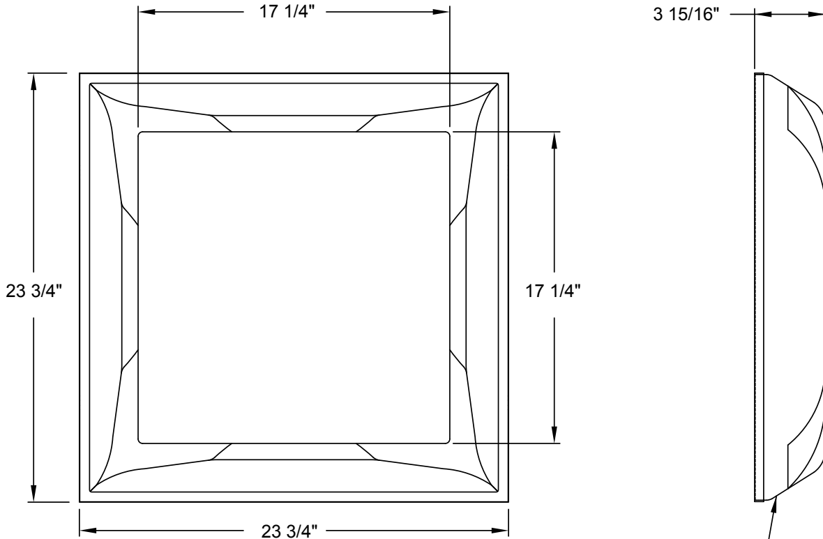
MOLDED R6 PLENUM (PRESCORED) CUT TO FIT COLLAR, 6", 8", 10", 12" & 14"
