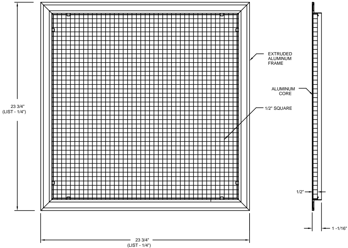
24" X 24" T-BAR SHOWN (overall 23 3/4 X 23 3/4") for 24" X 24" opening
