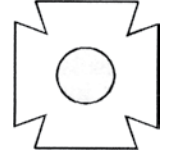
FIG. 4 Flashing w/ slit corners for crowned chimneys
